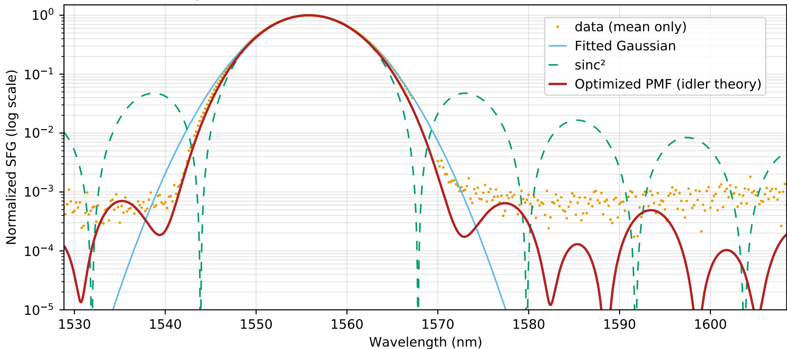
Four-step BG-removed Normalized SFG vs Wavelength (C+L, Log scale) \mu=1555.854 nm, FWHM=10.608 nm (CPKTP PMF overlaid)
